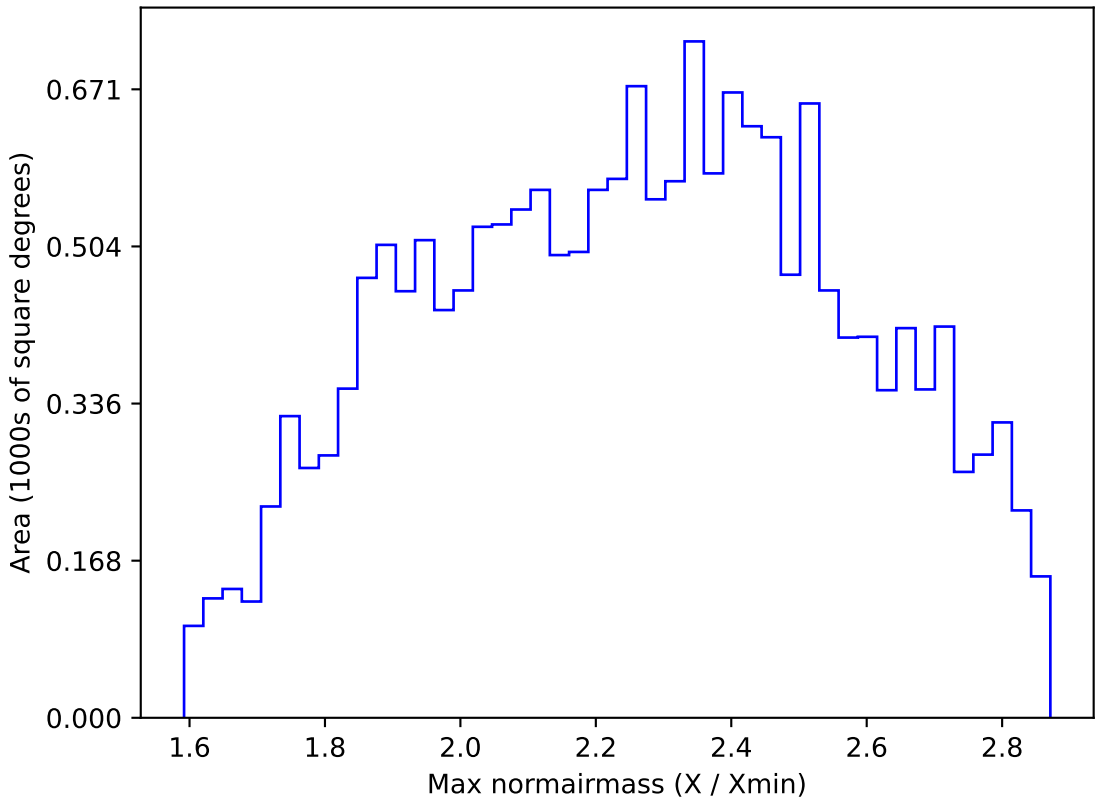
weather_cloudso0v3.5_10yrs WFD i band: Max normairmass
