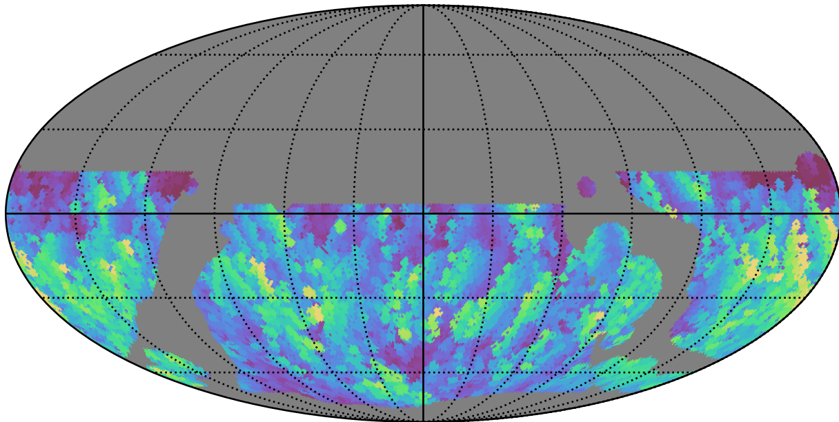
weather_cloudso0v3.5_10yrs WFD g band: Max normairmass
