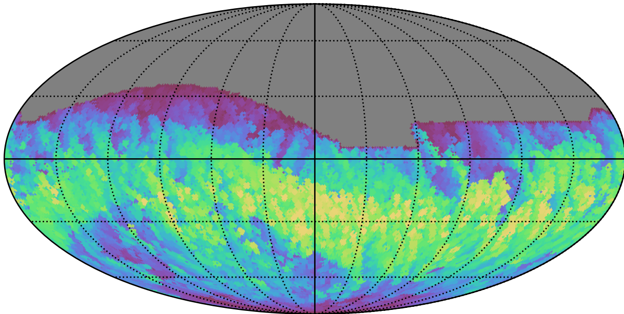
weather_cloudso0v3.5_10yrs All sky z band: Max normairmass
