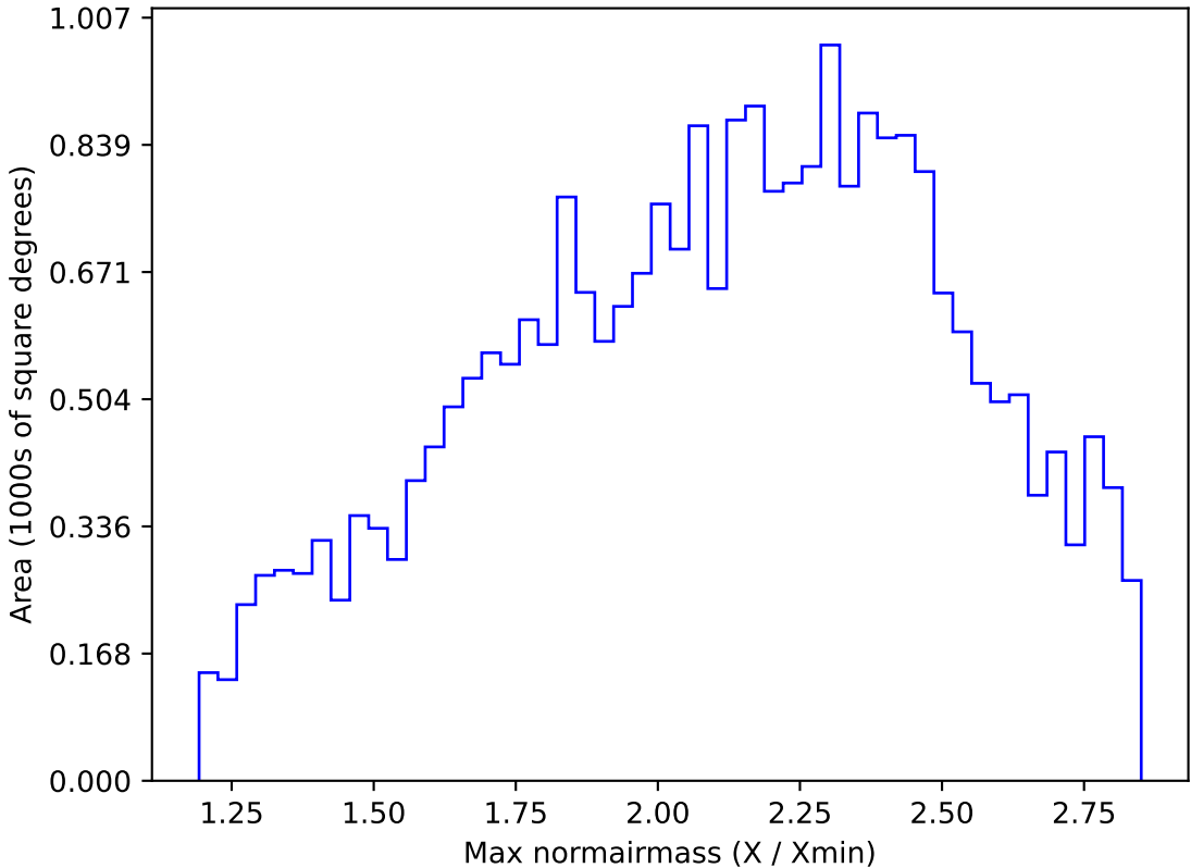
weather_cloudso0v3.5_10yrs All sky z band: Max normairmass
