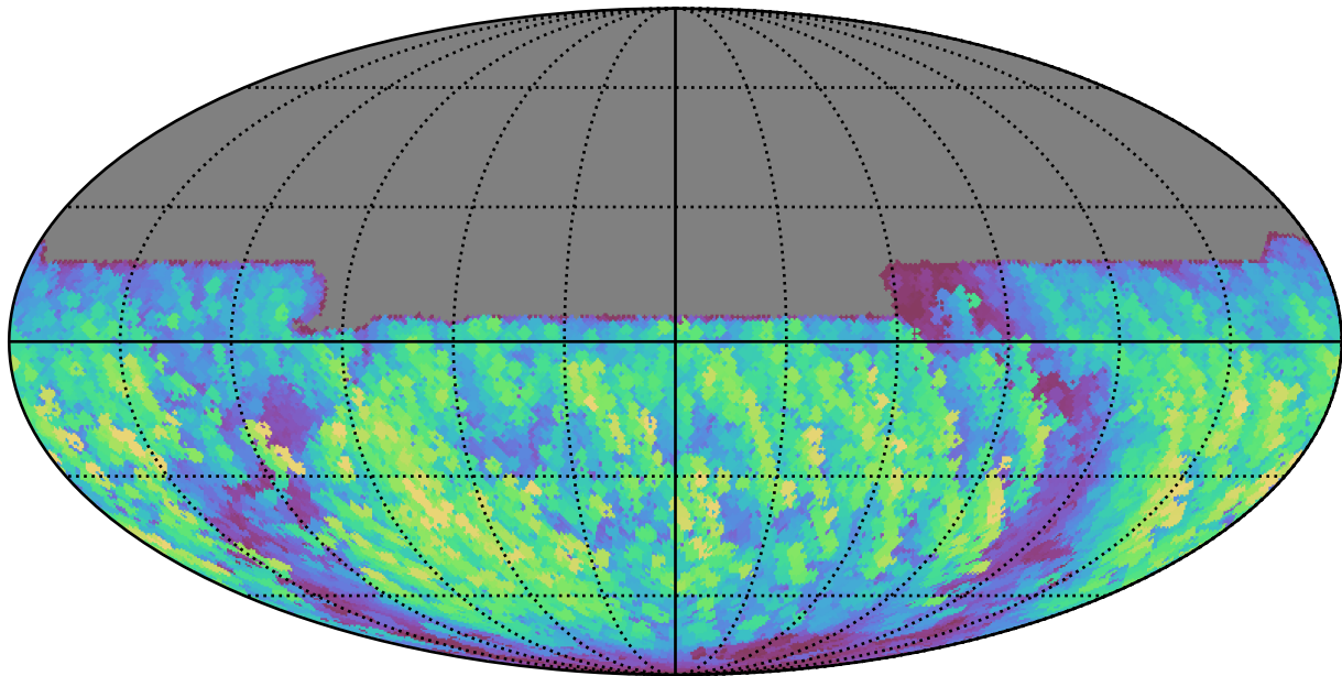
weather_cloudso0v3.5_10yrs All sky y band: Max normairmass
