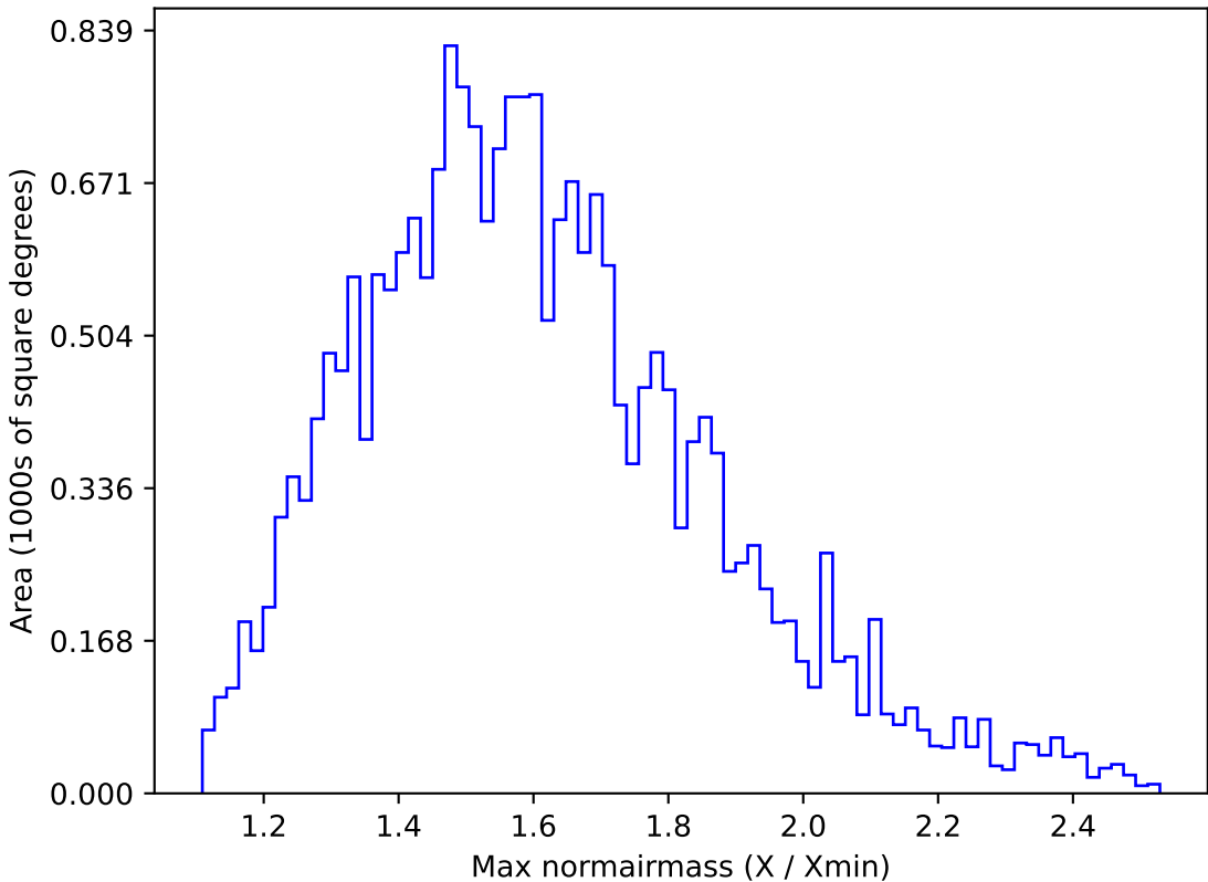
weather_cloudso0v3.5_10yrs All sky u band: Max normairmass
