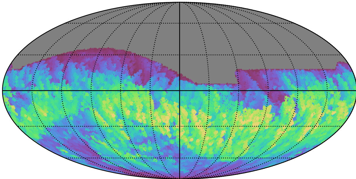
weather_cloudso0v3.5_10yrs All sky r band: Max normairmass
