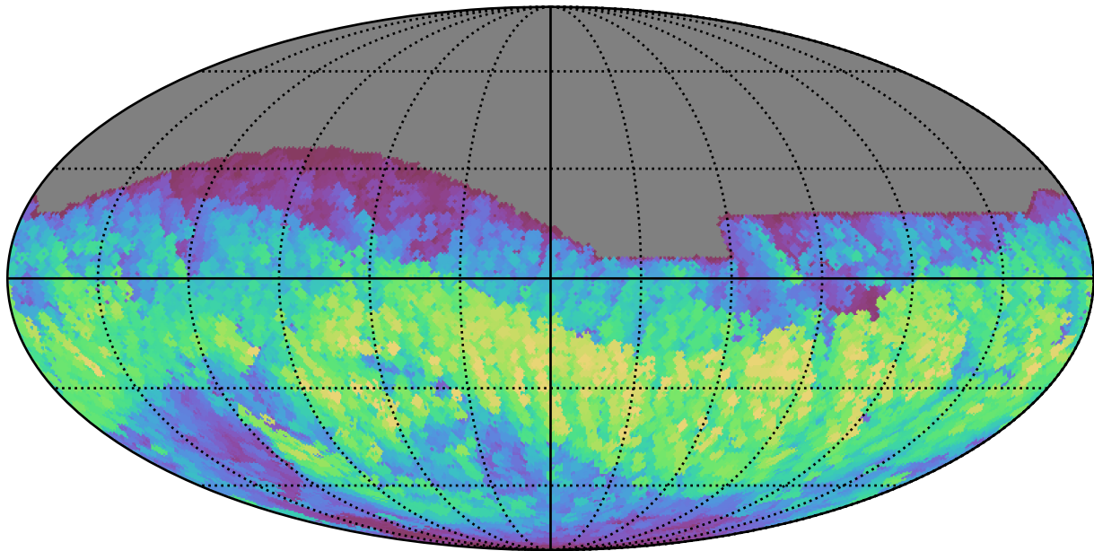
weather_cloudso0v3.5_10yrs All sky i band: Max normairmass
