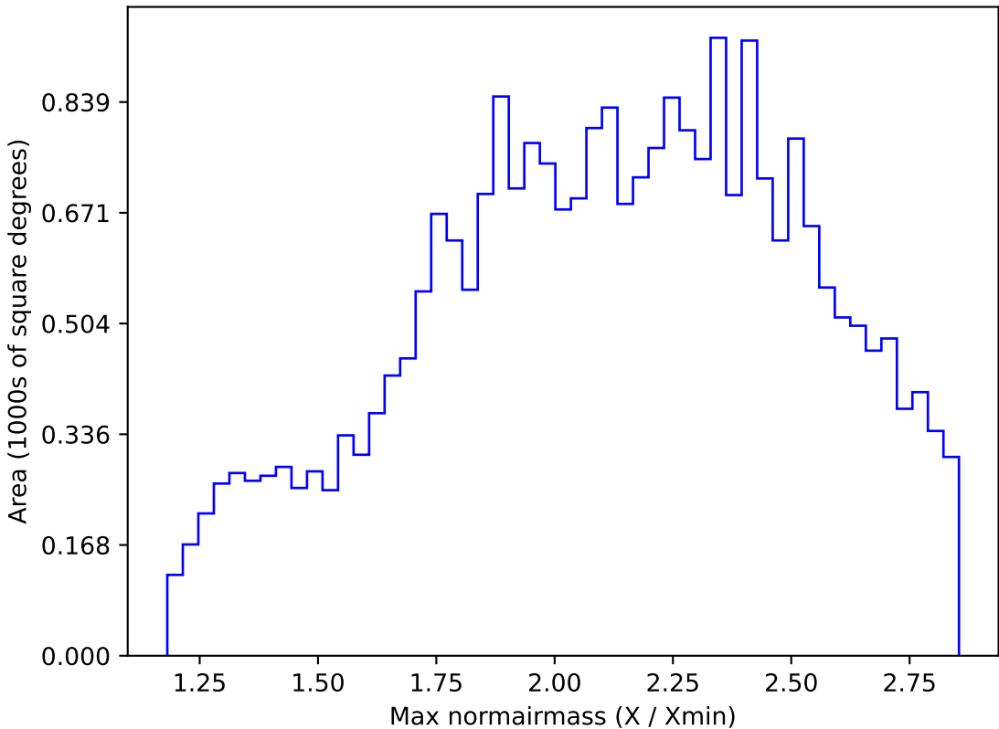
weather_cloudso0v3.5_10yrs All sky i band: Max normairmass
