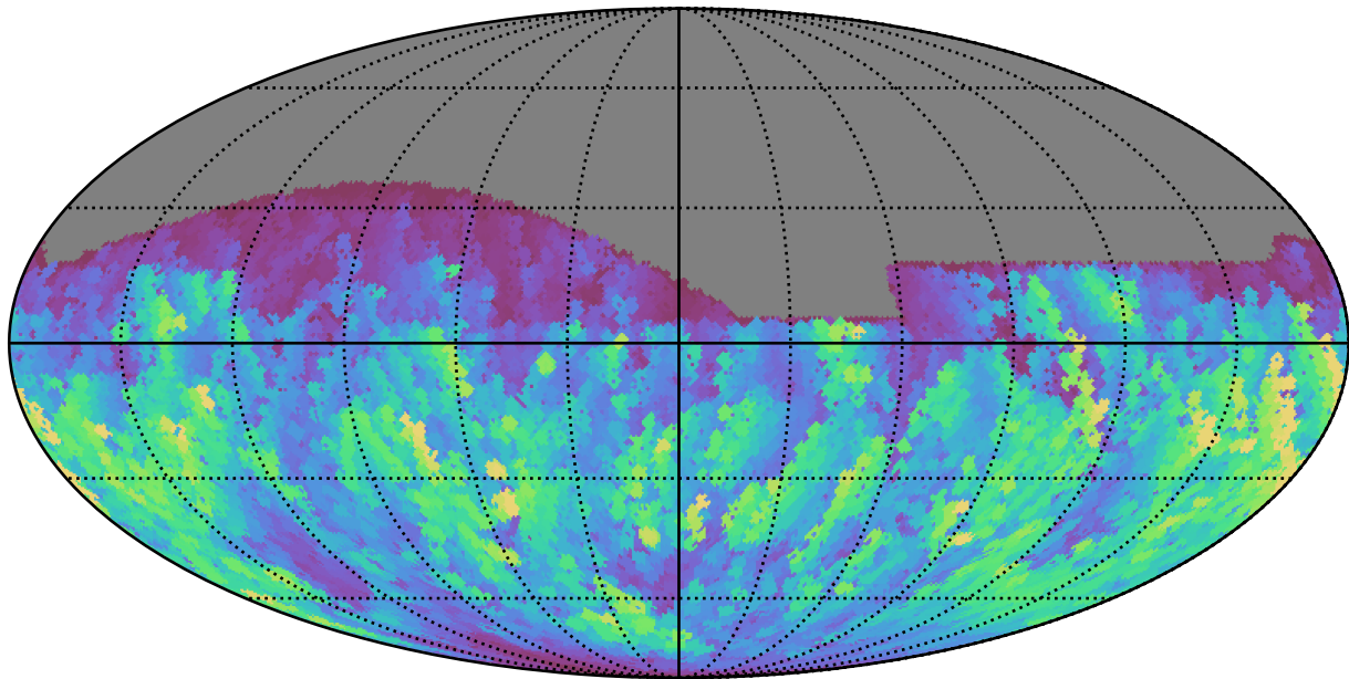
weather_cloudso0v3.5_10yrs All sky g band: Max normairmass
