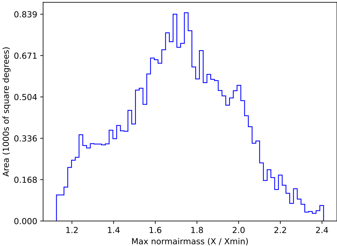
weather_cloudso0v3.5_10yrs All sky g band: Max normairmass
