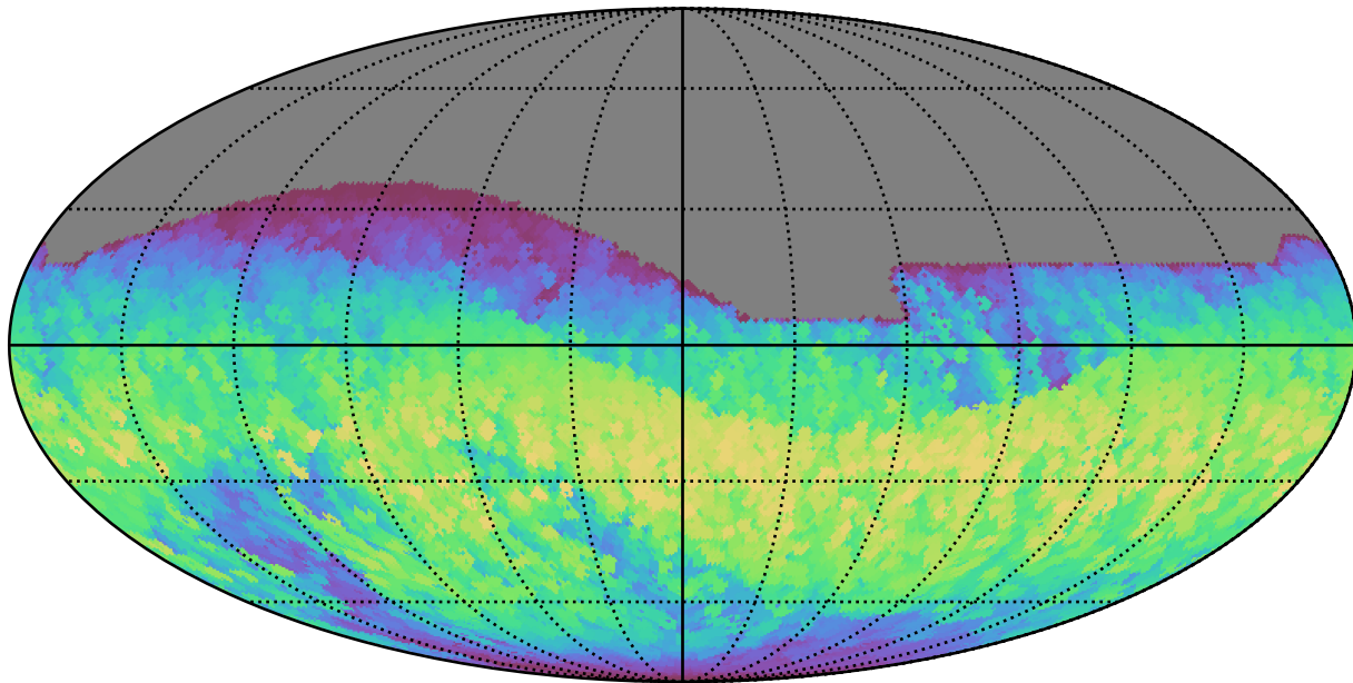
weather_cloudso0v3.5_10yrs All sky all bands: Max normairmass
