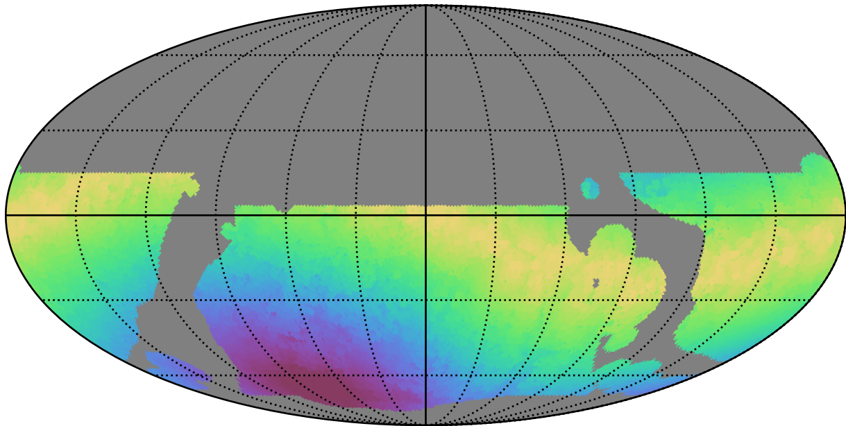
weather_cloudso0v3.5_10yrs WFD z band: Max moonDistance
