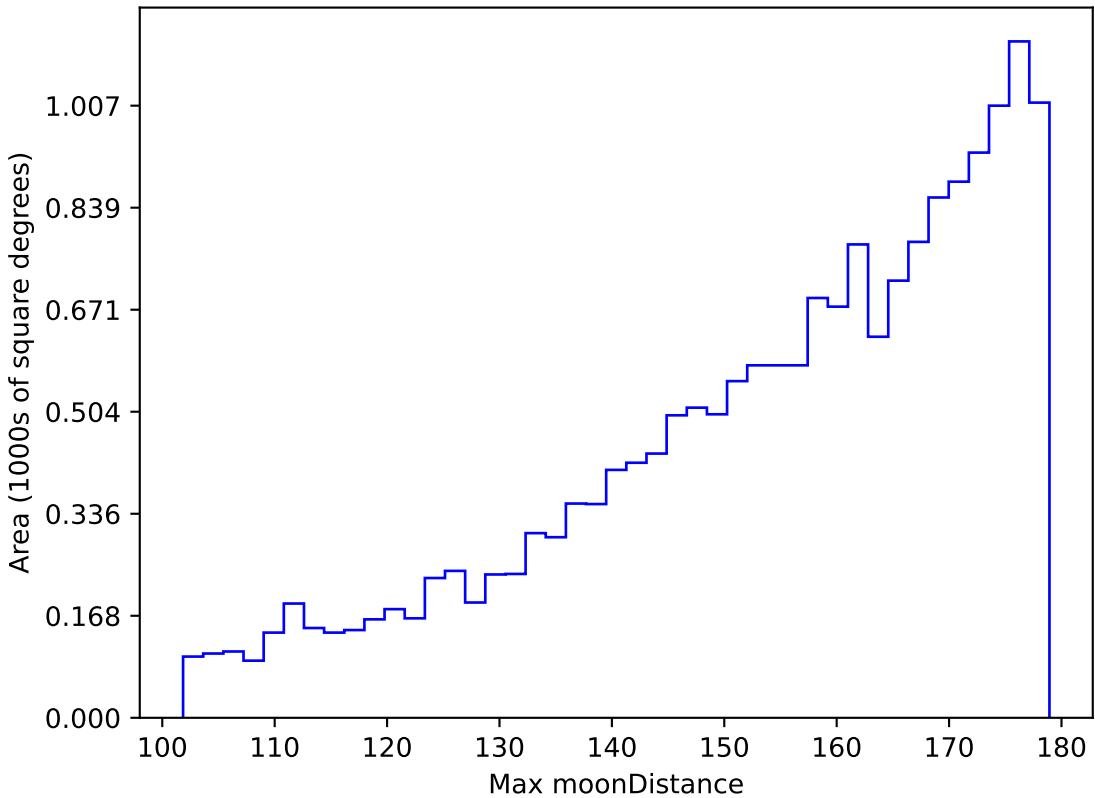
weather_cloudso0v3.5_10yrs WFD z band: Max moonDistance
