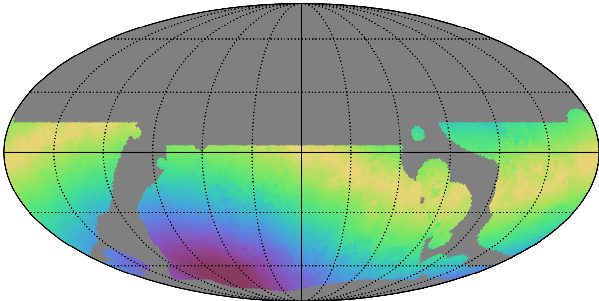
weather_cloudso0v3.5_10yrs WFD u band: Max moonDistance
