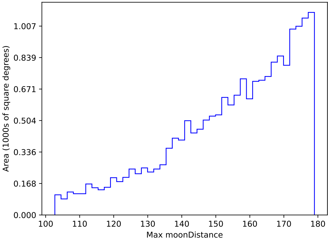
weather_cloudso0v3.5_10yrs WFD u band: Max moonDistance
