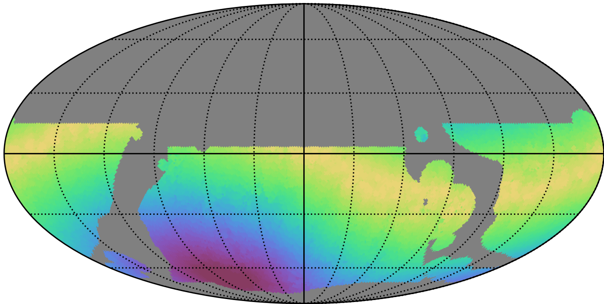
weather_cloudso0v3.5_10yrs WFD i band: Max moonDistance
