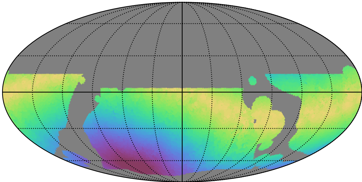
weather_cloudso0v3.5_10yrs WFD g band: Max moonDistance
