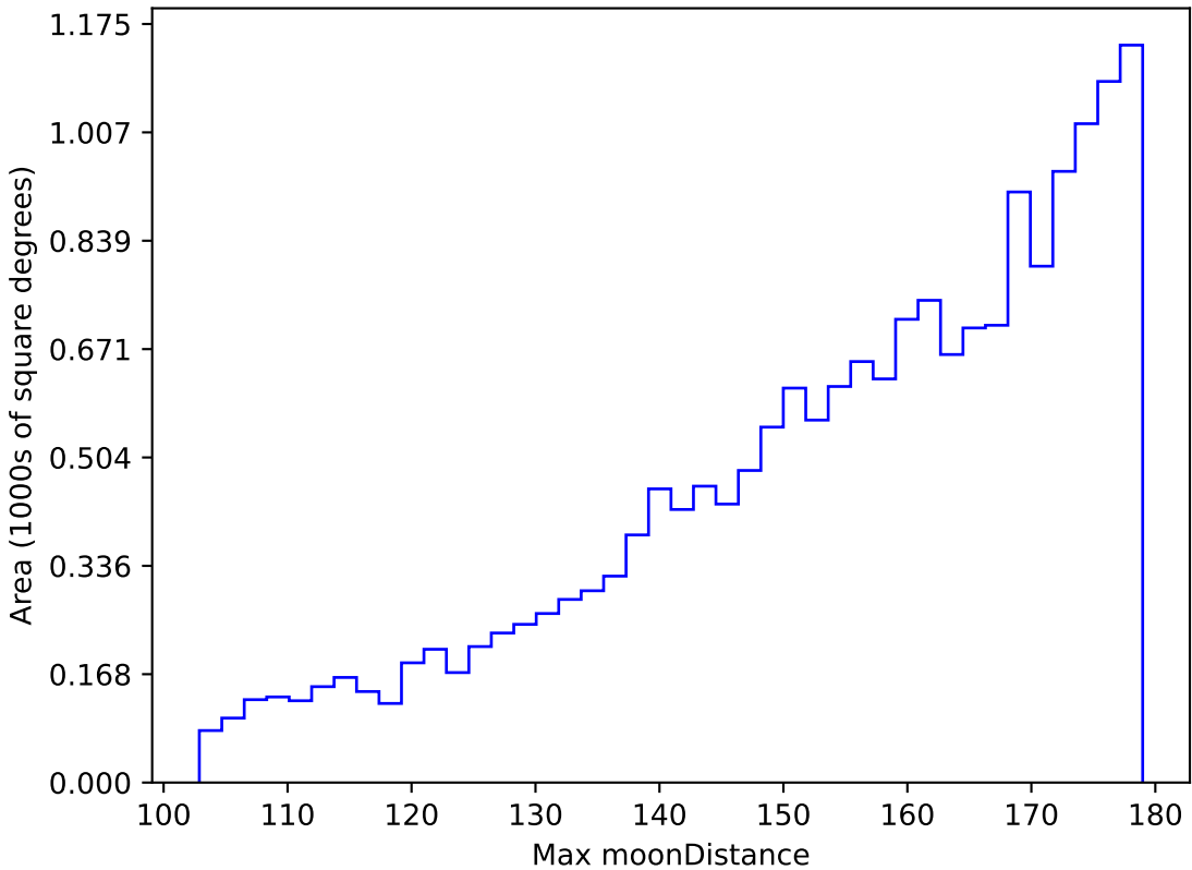
weather_cloudso0v3.5_10yrs WFD g band: Max moonDistance
