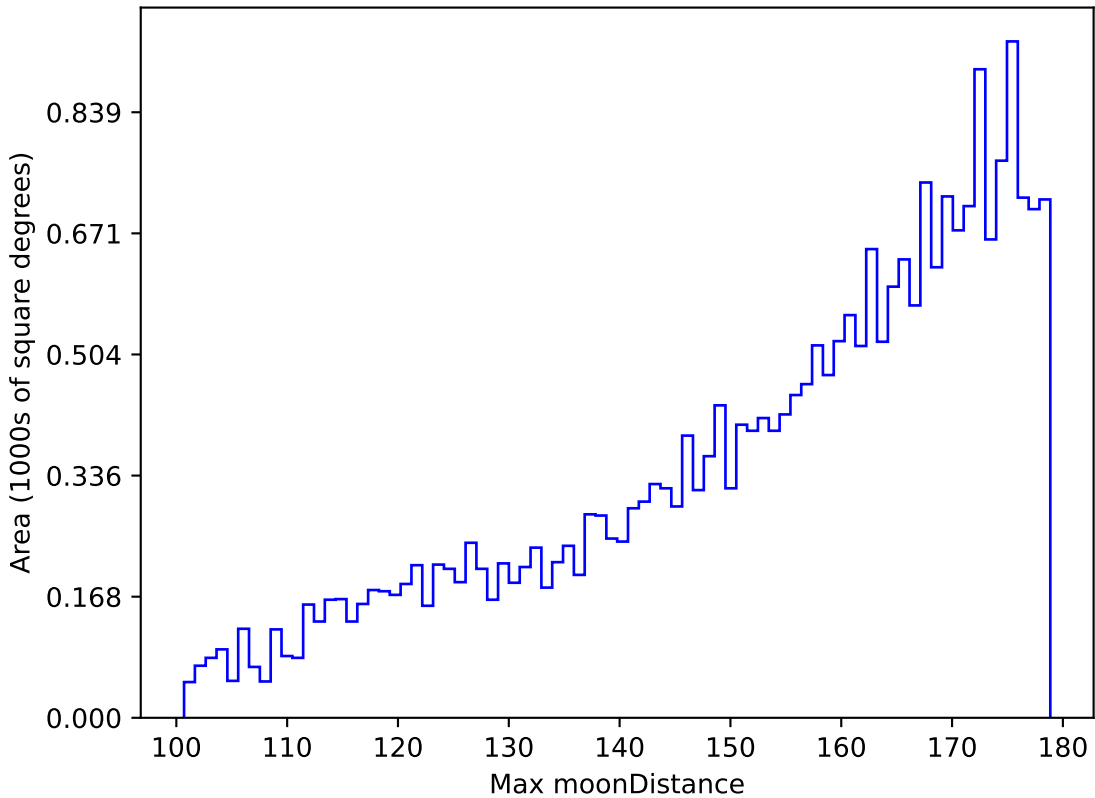
weather_cloudso0v3.5_10yrs All sky z band: Max moonDistance
