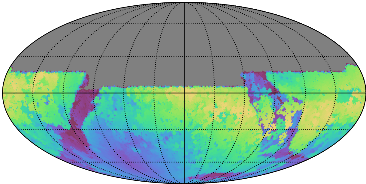
weather_cloudso0v3.5_10yrs All sky y band: Max moonDistance
