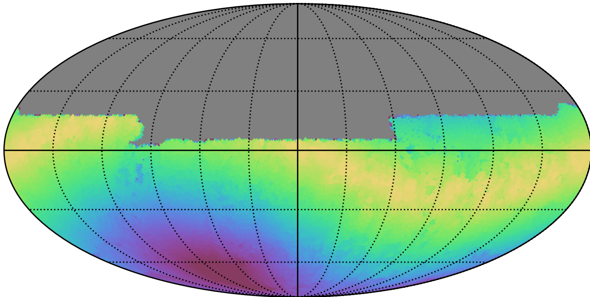
weather_cloudso0v3.5_10yrs All sky u band: Max moonDistance
