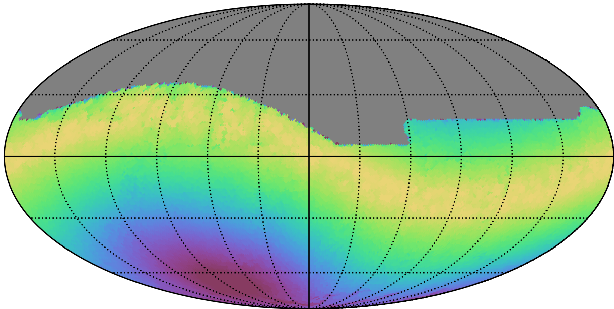
weather_cloudso0v3.5_10yrs All sky r band: Max moonDistance
