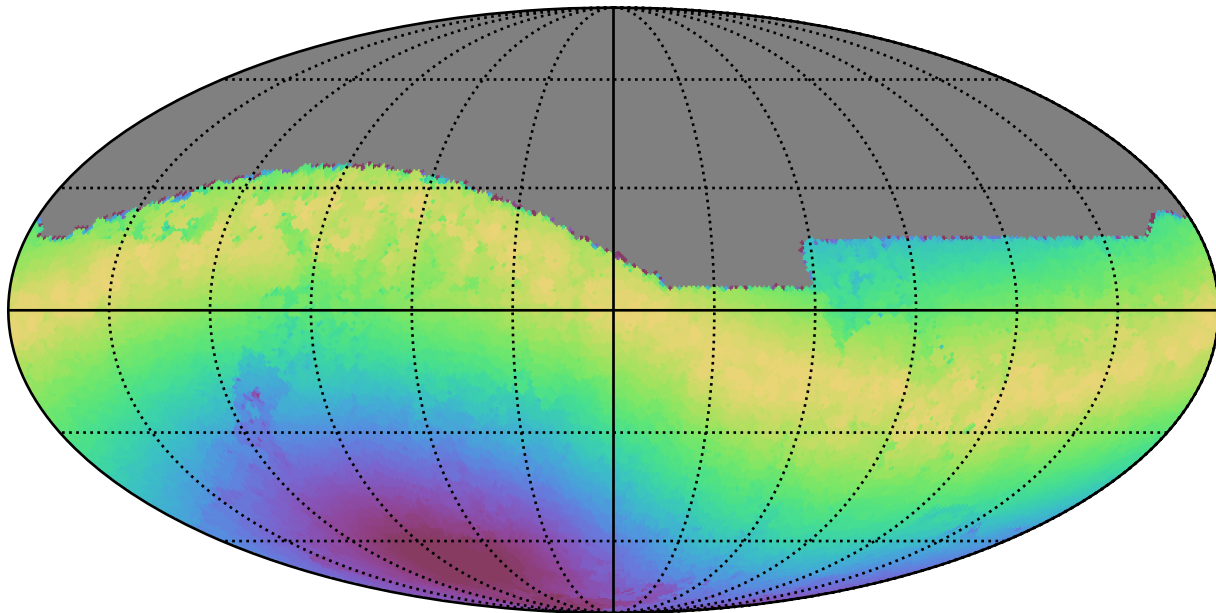
weather_cloudso0v3.5_10yrs All sky i band: Max moonDistance
