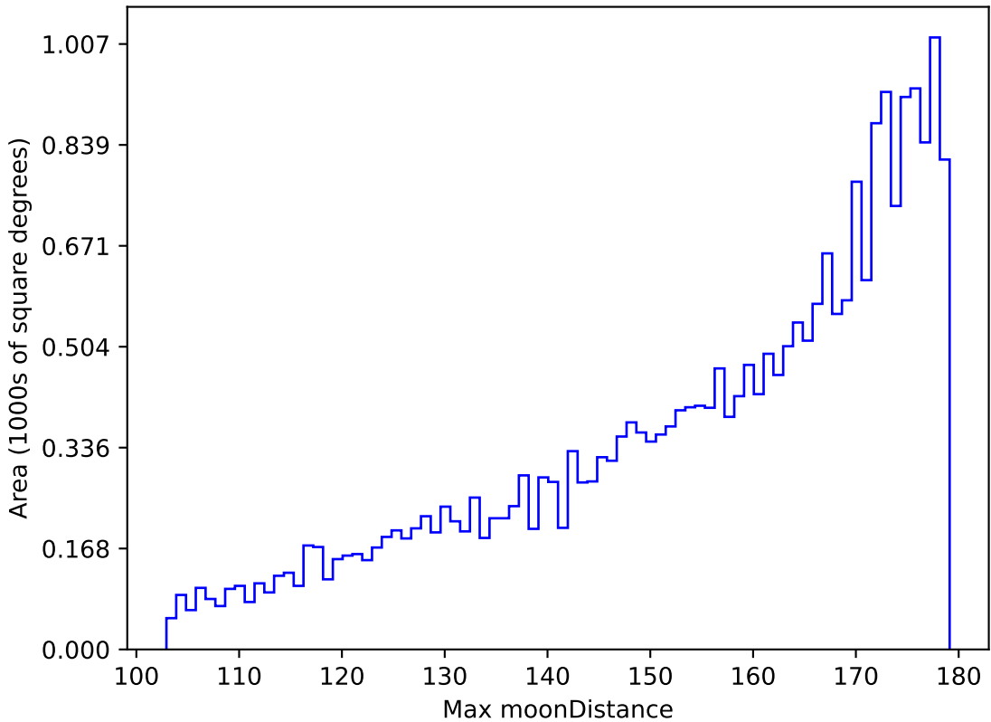
weather_cloudso0v3.5_10yrs All sky i band: Max moonDistance
