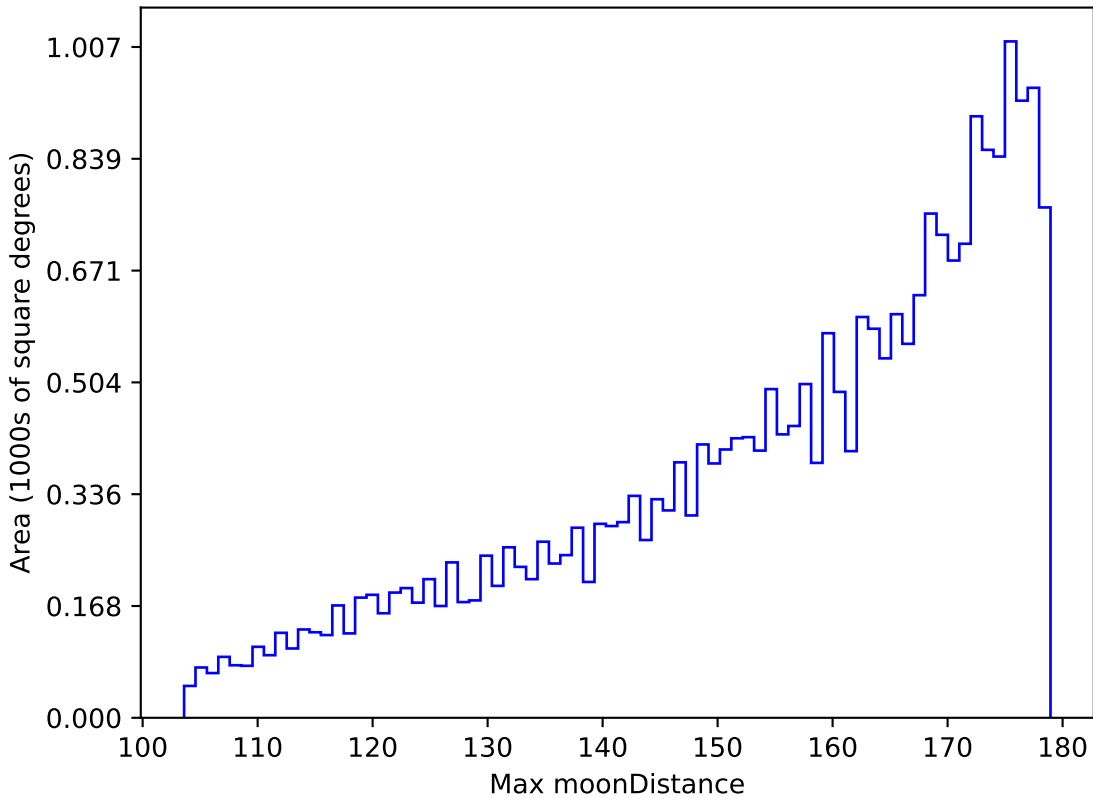
weather_cloudso0v3.5_10yrs All sky g band: Max moonDistance
