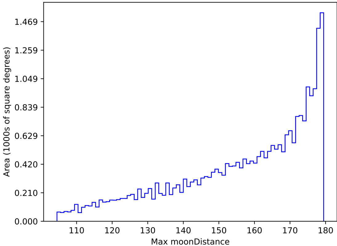
weather_cloudso0v3.5_10yrs All sky all bands: Max moonDistance
