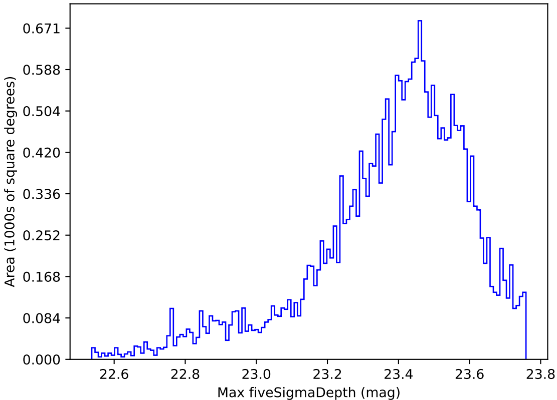
weather_cloudso0v3.5_10yrs Yr 1 z band: Max fiveSigmaDepth
