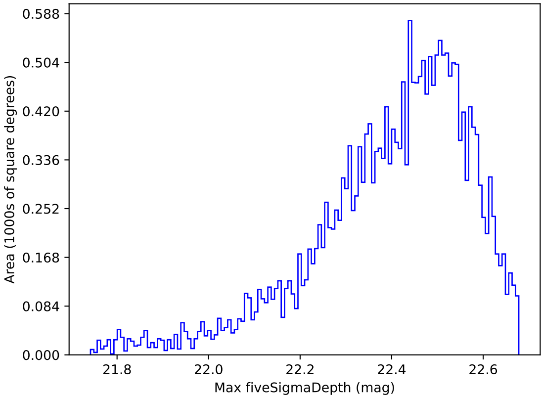
weather_cloudso0v3.5_10yrs Yr 1 y band: Max fiveSigmaDepth
