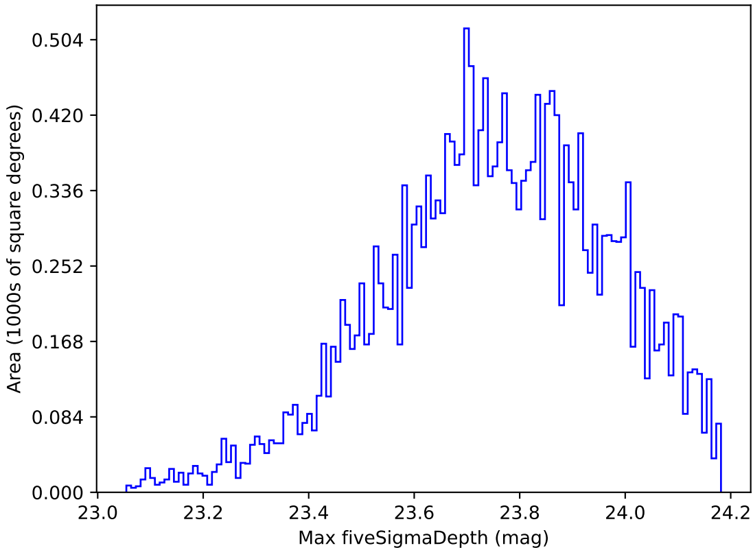
weather_cloudso0v3.5_10yrs Yr 1 u band: Max fiveSigmaDepth
