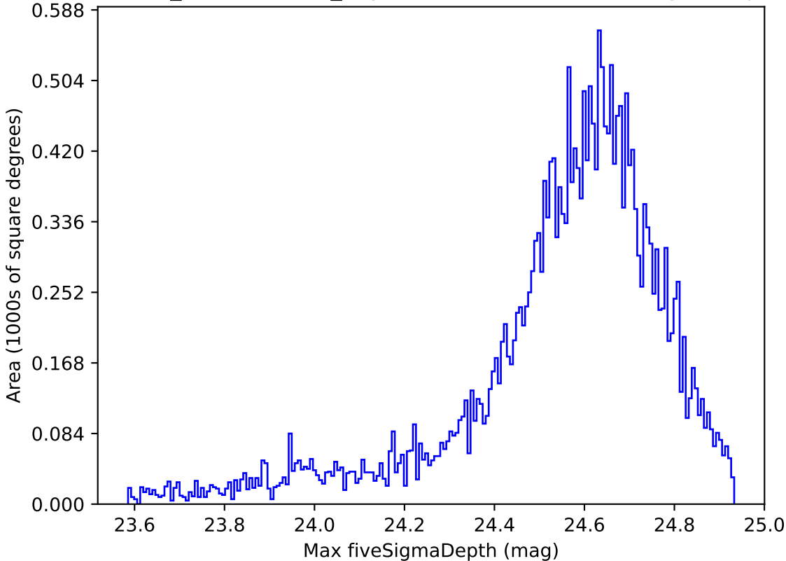
weather_cloudso0v3.5_10yrs Yr 1 r band: Max fiveSigmaDepth
