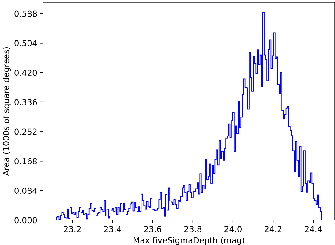
weather_cloudso0v3.5_10yrs Yr 1 i band: Max fiveSigmaDepth
