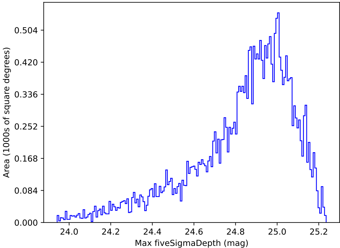
weather_cloudso0v3.5_10yrs Yr 1 g band: Max fiveSigmaDepth
