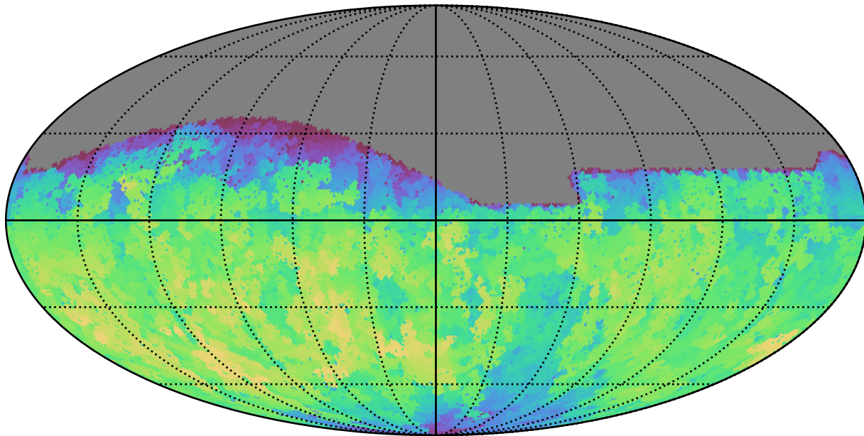
weather_cloudso0v3.5_10yrs Yr 1 all bands: Max fiveSigmaDepth
