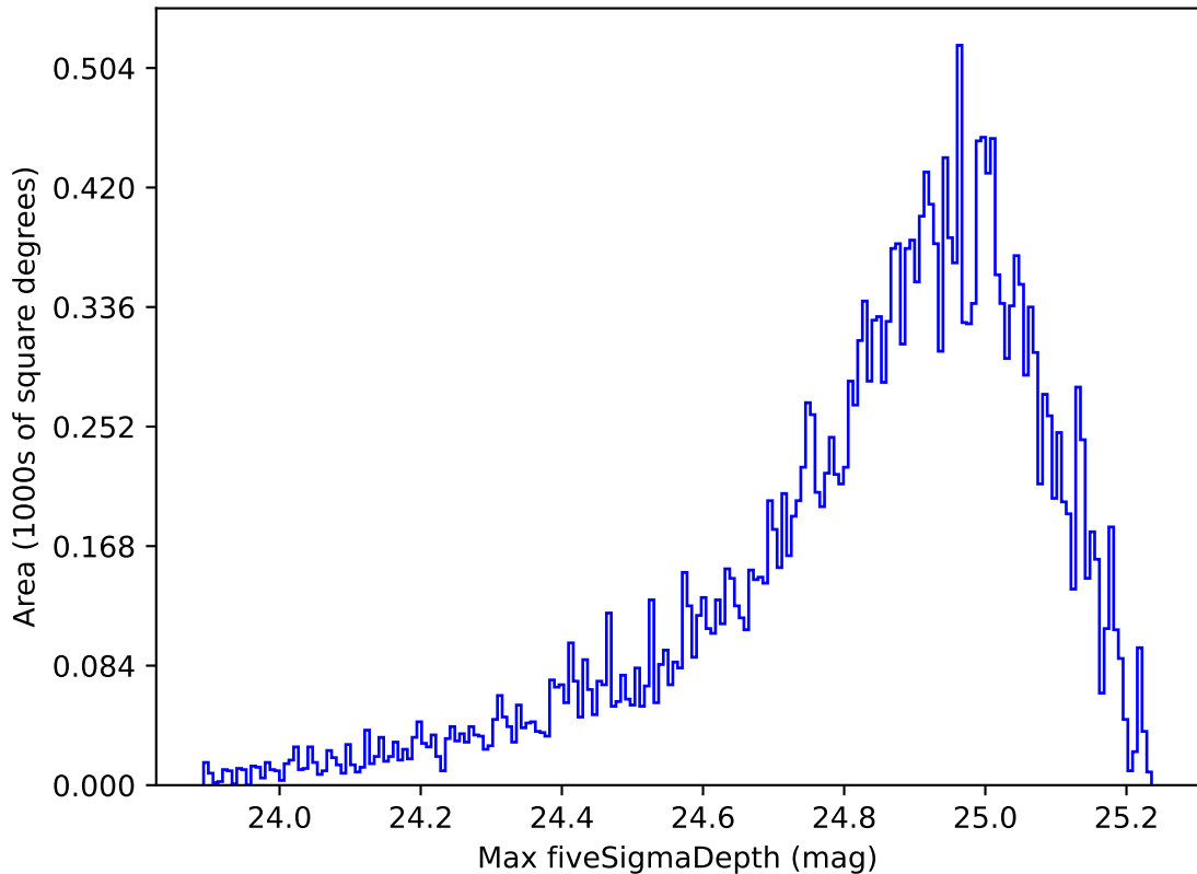
weather_cloudso0v3.5_10yrs Yr 1 all bands: Max fiveSigmaDepth
