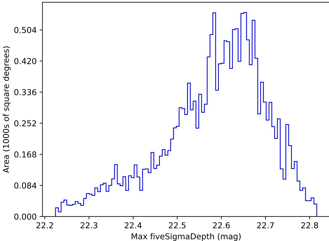
weather_cloudso0v3.5_10yrs WFD y band: Max fiveSigmaDepth
