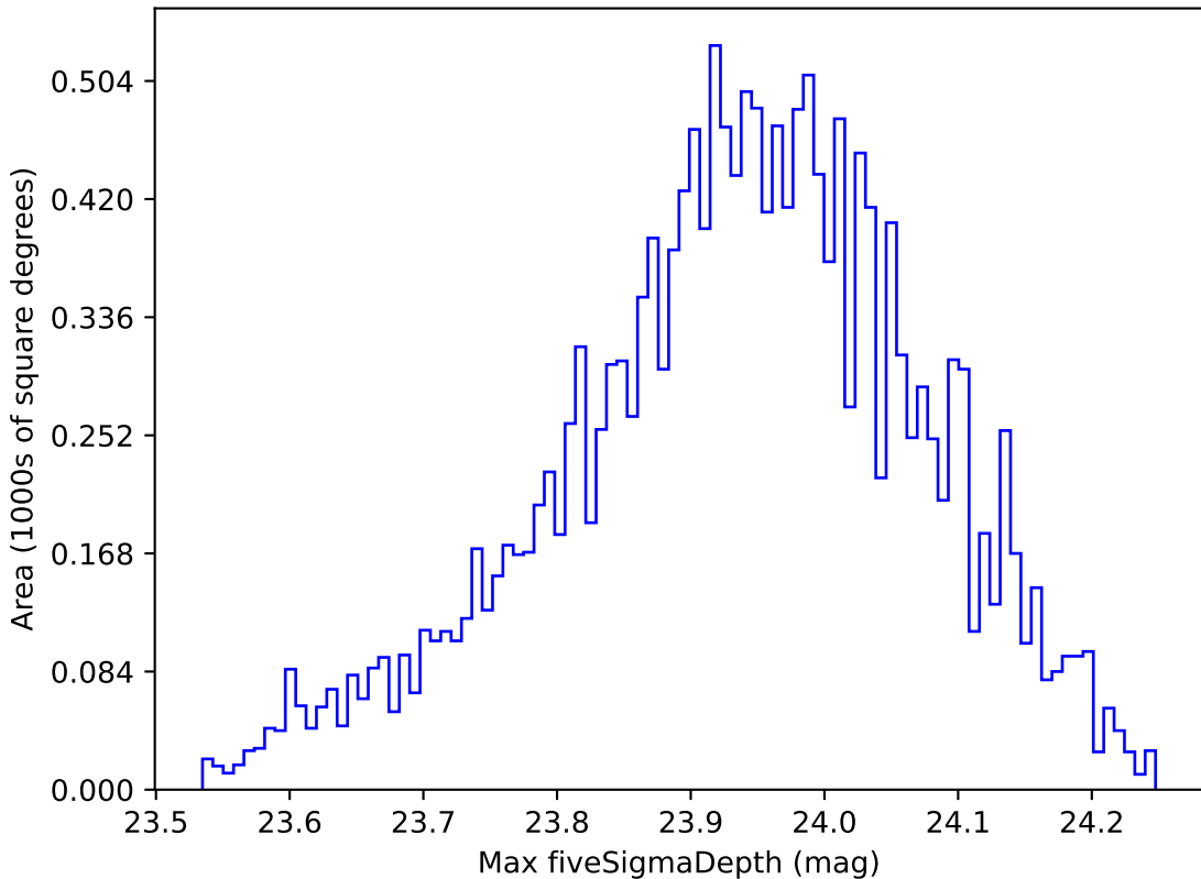
weather_cloudso0v3.5_10yrs WFD u band: Max fiveSigmaDepth
