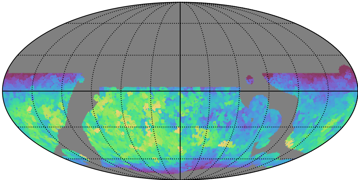
weather_cloudso0v3.5_10yrs WFD r band: Max fiveSigmaDepth
