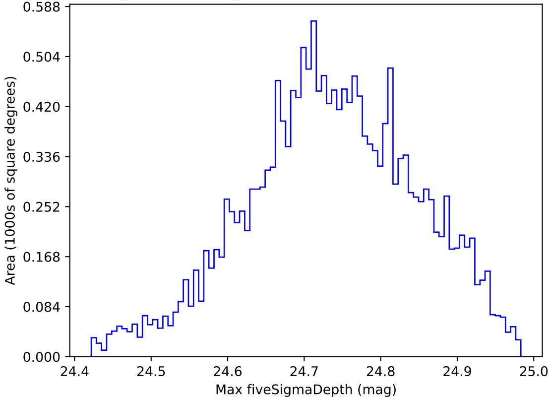
weather_cloudso0v3.5_10yrs WFD r band: Max fiveSigmaDepth
