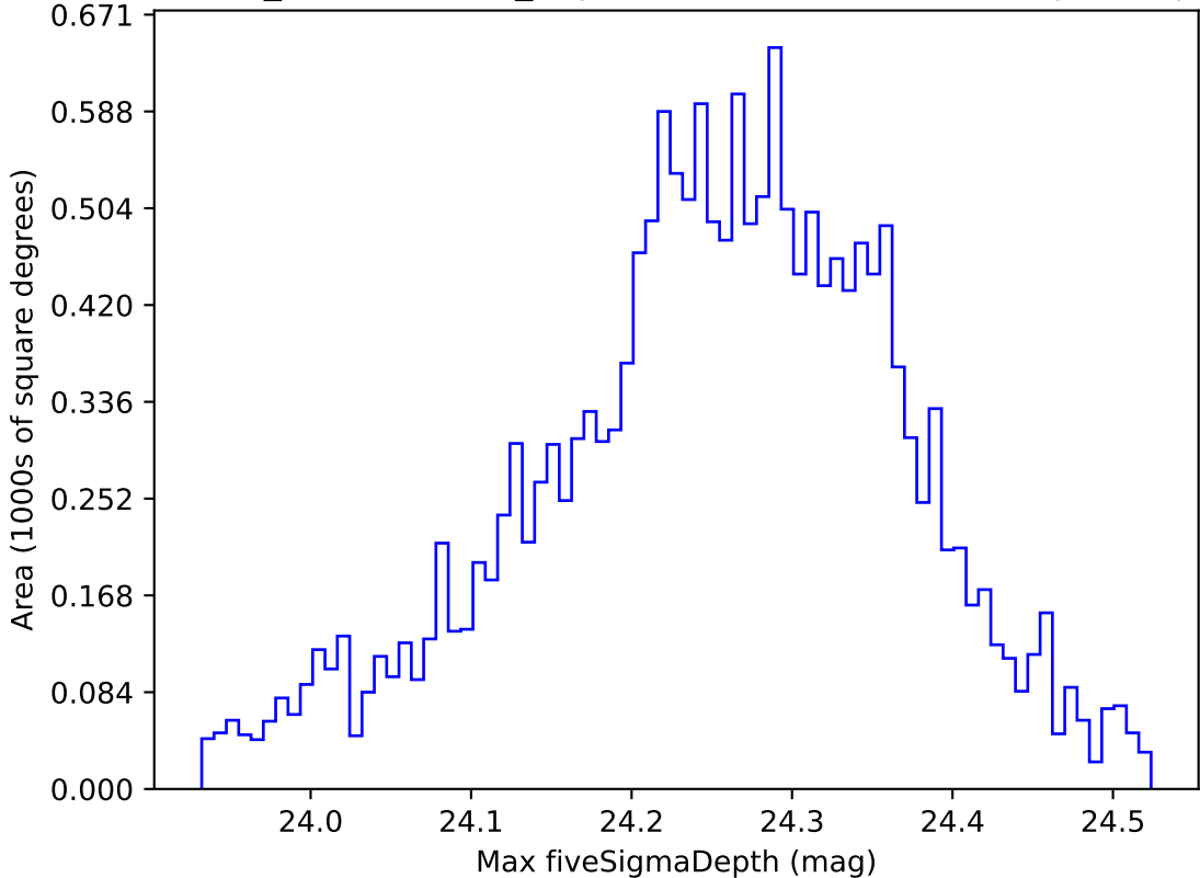
weather_cloudso0v3.5_10yrs WFD i band: Max fiveSigmaDepth
