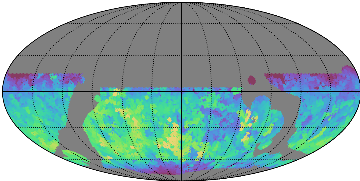
weather_cloudso0v3.5_10yrs WFD g band: Max fiveSigmaDepth
