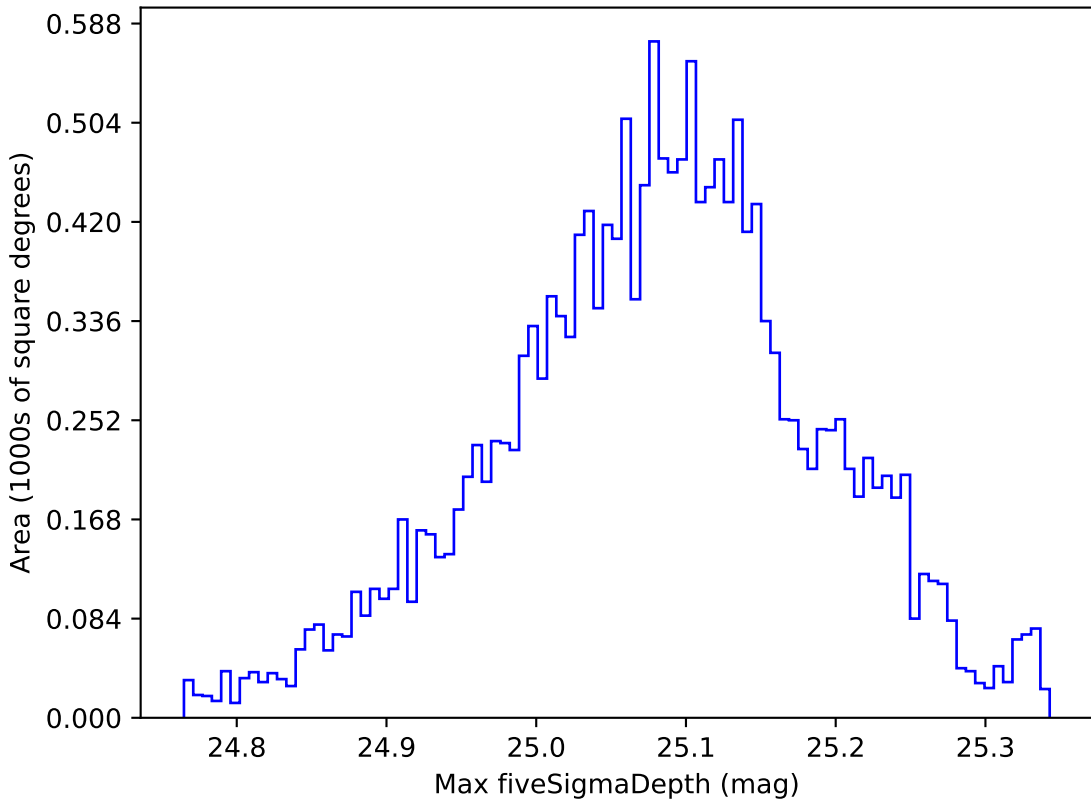
weather_cloudso0v3.5_10yrs WFD g band: Max fiveSigmaDepth
