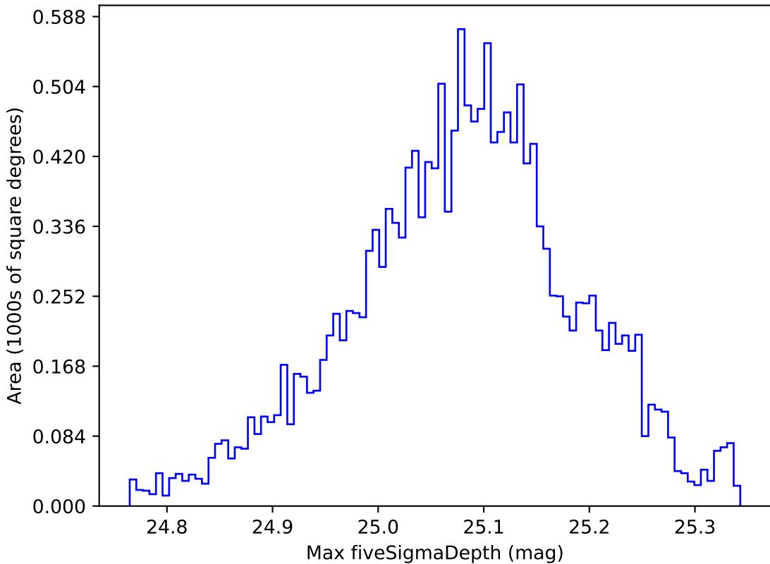
weather_cloudso0v3.5_10yrs WFD all bands: Max fiveSigmaDepth
