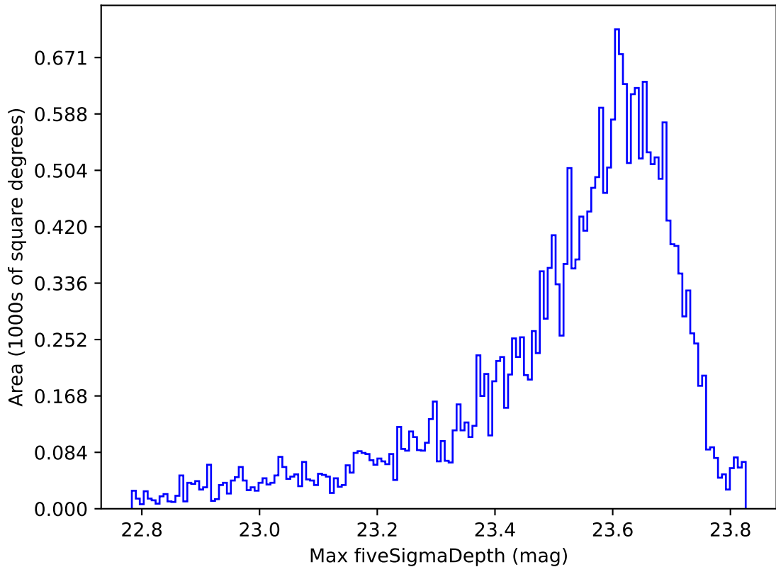
weather_cloudso0v3.5_10yrs All sky z band: Max fiveSigmaDepth
