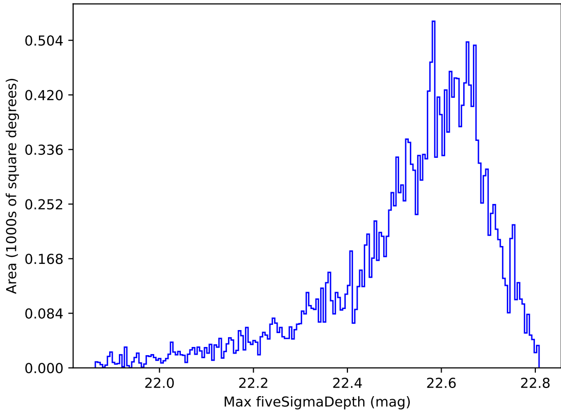
weather_cloudso0v3.5_10yrs All sky y band: Max fiveSigmaDepth
