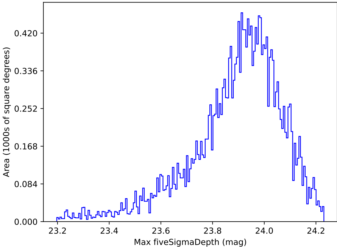
weather_cloudso0v3.5_10yrs All sky u band: Max fiveSigmaDepth
