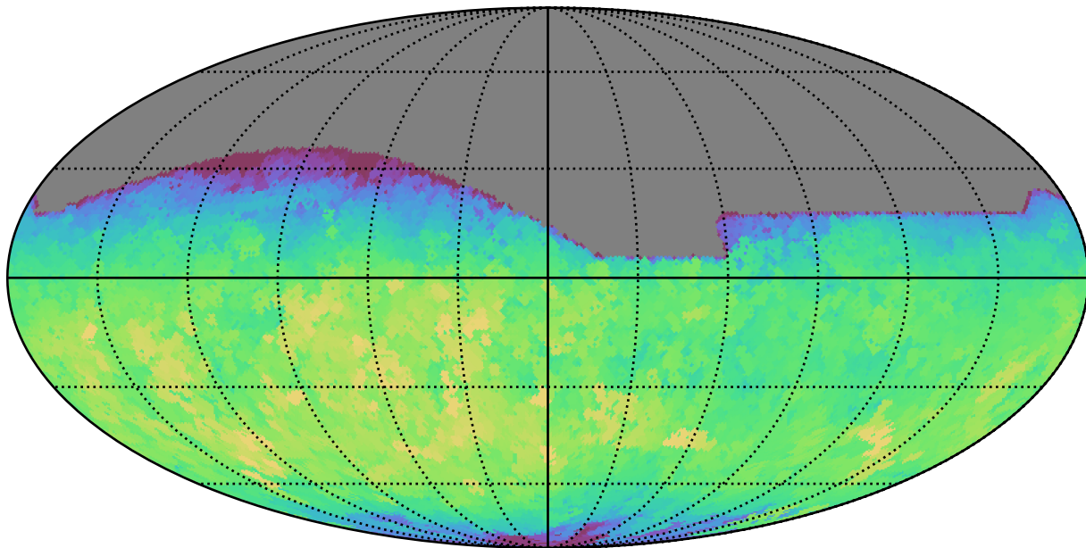
weather_cloudso0v3.5_10yrs All sky r band: Max fiveSigmaDepth
