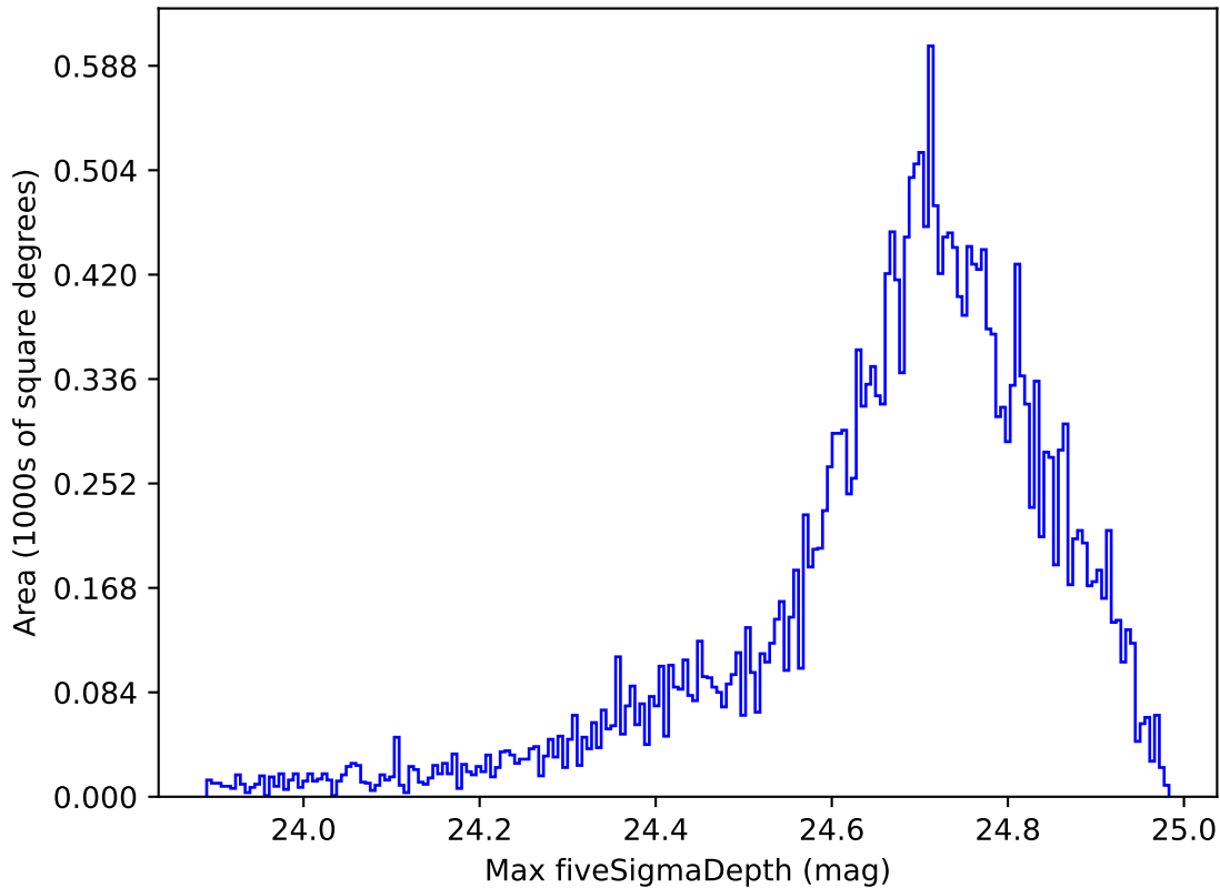
weather_cloudso0v3.5_10yrs All sky r band: Max fiveSigmaDepth
