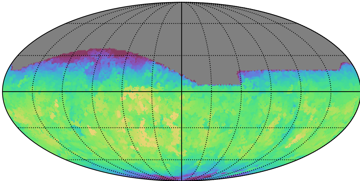
weather_cloudso0v3.5_10yrs All sky i band: Max fiveSigmaDepth
