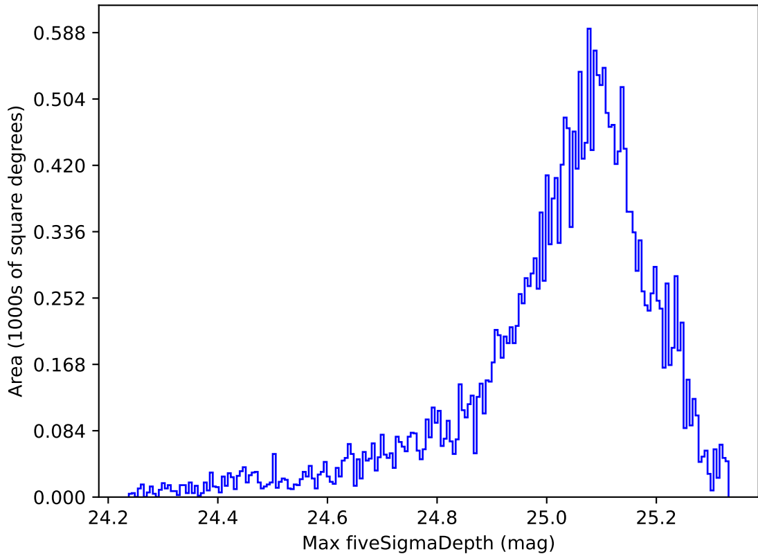
weather_cloudso0v3.5_10yrs All sky g band: Max fiveSigmaDepth
